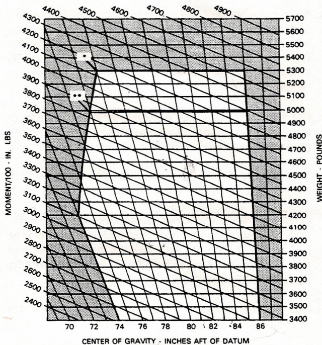
MOMENT LIMIT vs WEIGHT
